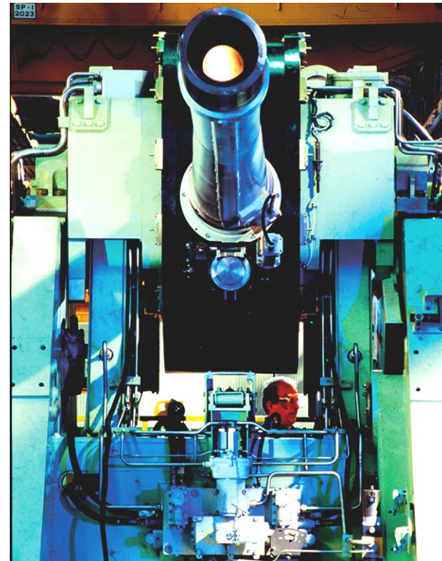
127/64 RECOILING MASS
